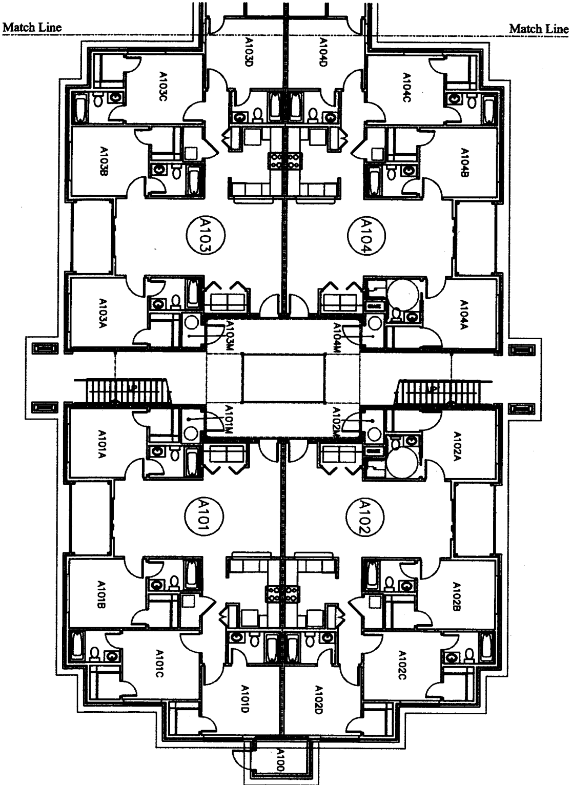
Building "A" - First Floor Plan-North End
