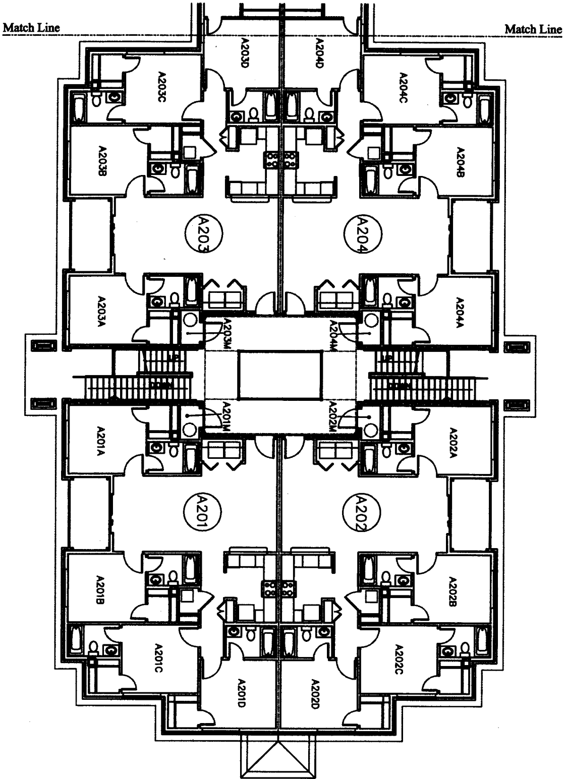
Building "A" - Second Floor Plan-North End
