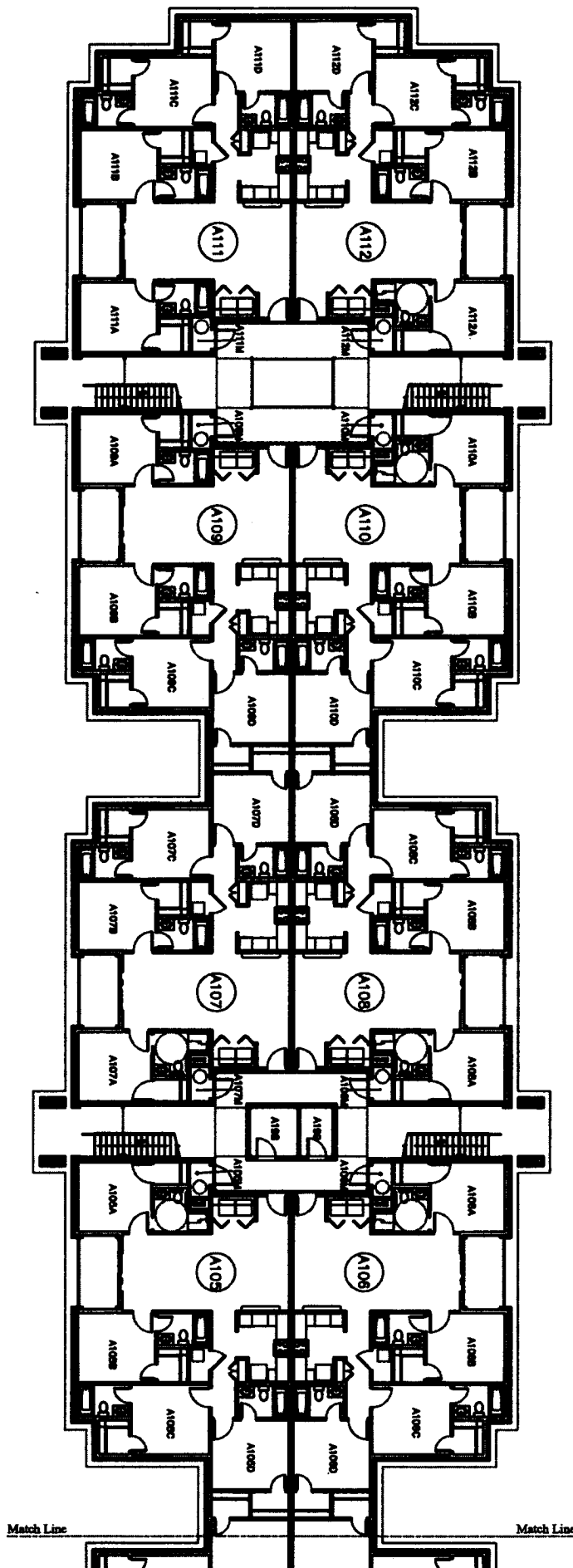
Building "A" - First Floor Plan-South End NOT TO SCALE
