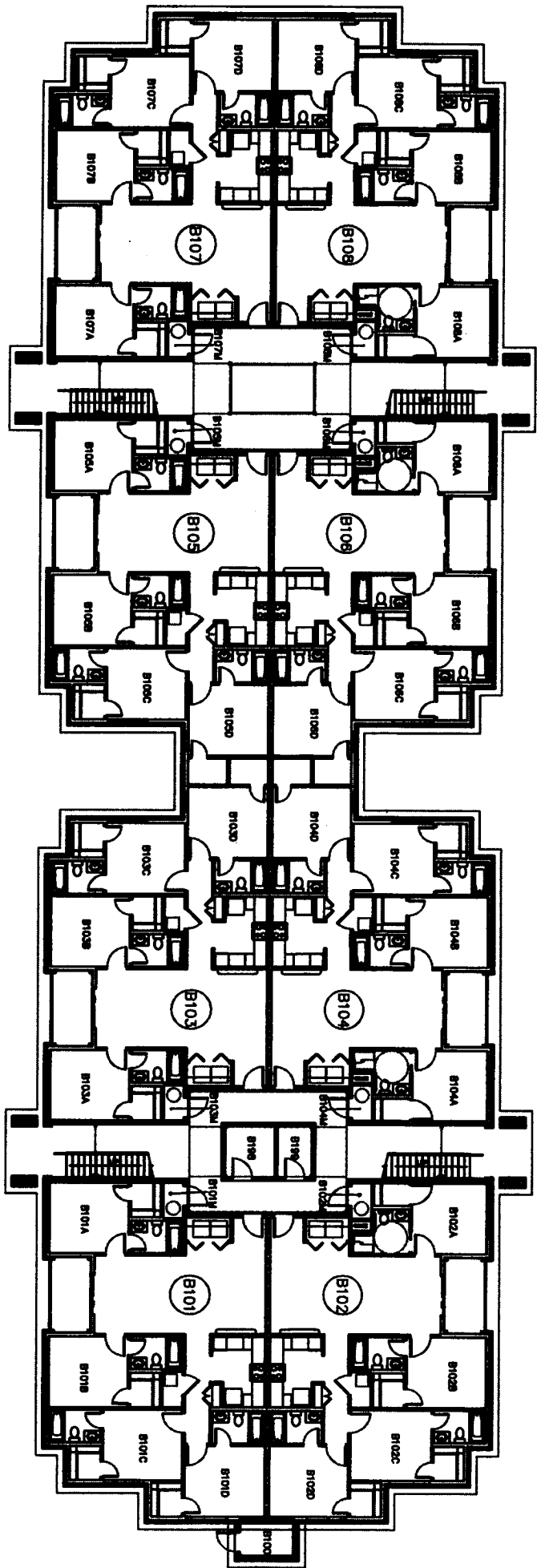
Building "B" - First Floor Plan NOT TO SCALE
